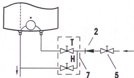
The "above-supply-point" version
