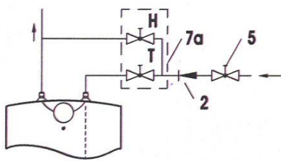
The "below-supply-point" version
