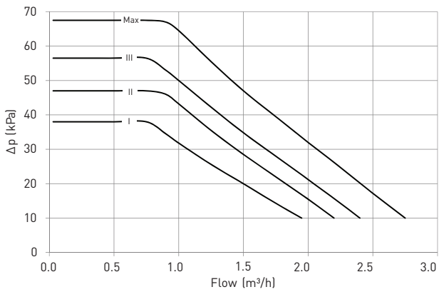
PUMP CHARACTERISTICS, UPM3 AUTO L
