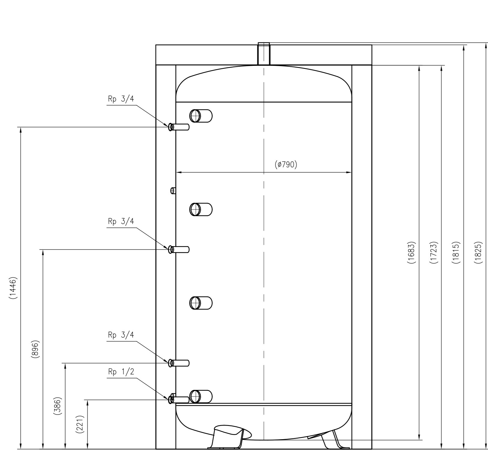
Side view
