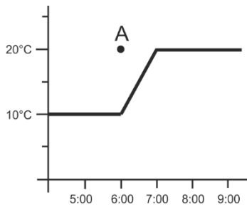
Room temperature - OPTIMUM START OFF
